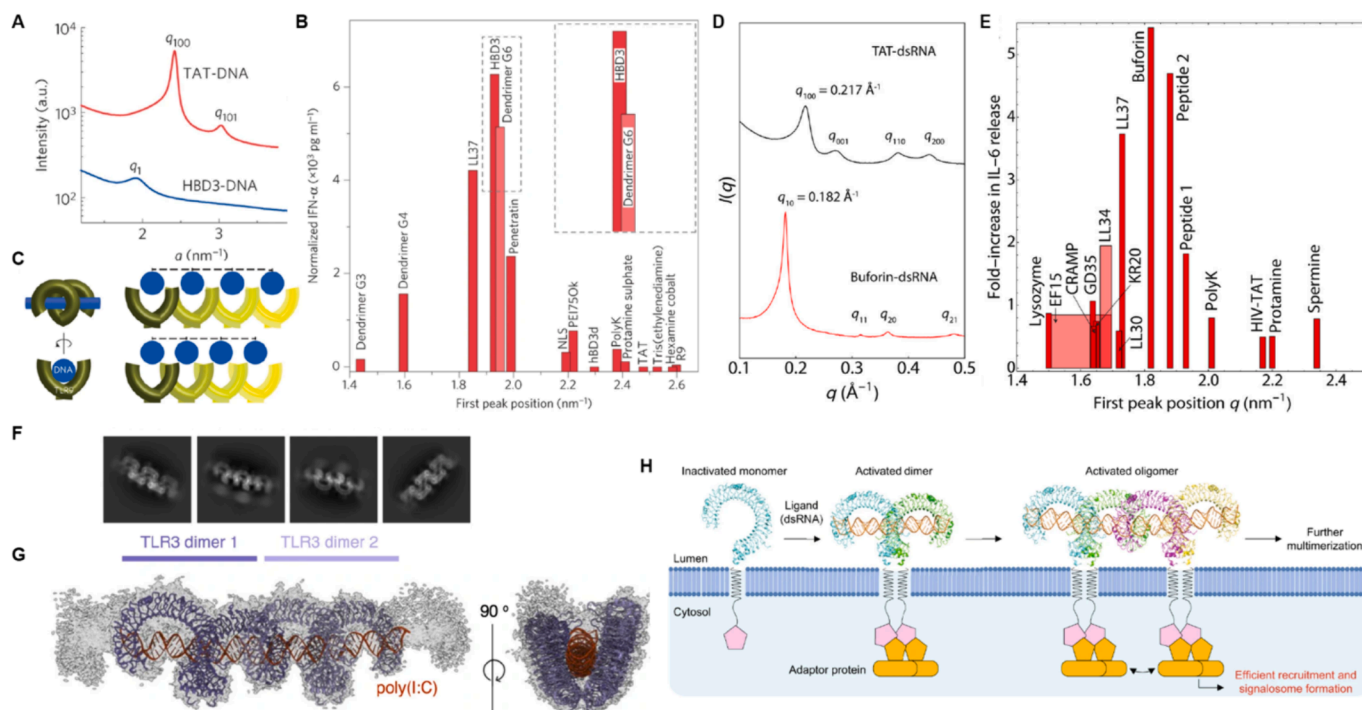
Fig. 2. Inter-nucleic acid spacing in the polycation-nucleic acid complex strongly influences the amplitude of immune activation. (A) SAXS data from TAT-dsDNA complex and HBD-dsDNA complex. TAT organizes dsDNA into a 3D columnar hexagonal lattice with parameters a = 2.90 nm, c = 3.50 nm, while HBD organizes dsDNA into a disordered columnar lattice with an average inter-dsDNA distance as 3.25 nm. (B) IFN- \alpha production in human pDCs through TLR9 activation depends strongly on dsDNA spacing in paracrystalline dsDNA complexes formed with different polycations. (C) Side-on and end-on views of binding between a dsDNA complex and multiple TLR9 receptors. (panel A-C is adapted from reference [54]) (D) SAXS data obtained from TAT-dsRNA complex and buforin-dsRNA complex. TAT organizes dsRNA into a 3D hexagonal lattice with the inter-dsRNA spacing of \sim 2.90 nm. In comparison, buforin organizes dsRNA into a 2D hexagonal lattice with an inter-dsRNA spacing of 3.45 nm. (E) The amplitude of IL-6 release from the polycation-dsRNA complex-treated NHEK cells depends on the inter-dsRNA spacing. (Panels D and E are adapted from reference [53]) (F) Representative cryoEM images of multiple TLR3 monomer polymerize along the poly(I:C) chain, a synthetic analog of dsRNA. (G) Electron density map of the TLR3-poly(I:C) complex. (Panels F and G are adapted from reference [55]) (H) A schematic shows the polymerization of TLR3 along the ordered dsRNA chains induces stronger adaptor protein recruitment and activation. (scheme adapted from reference [56]).
