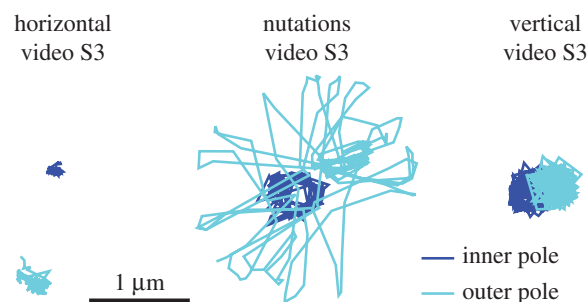
Figure 5. Position of poles during different behaviours observed in S. oneidensis . The poles are the foci of the fitted ellipses used in image analysis (see the electronic supplementary material).
